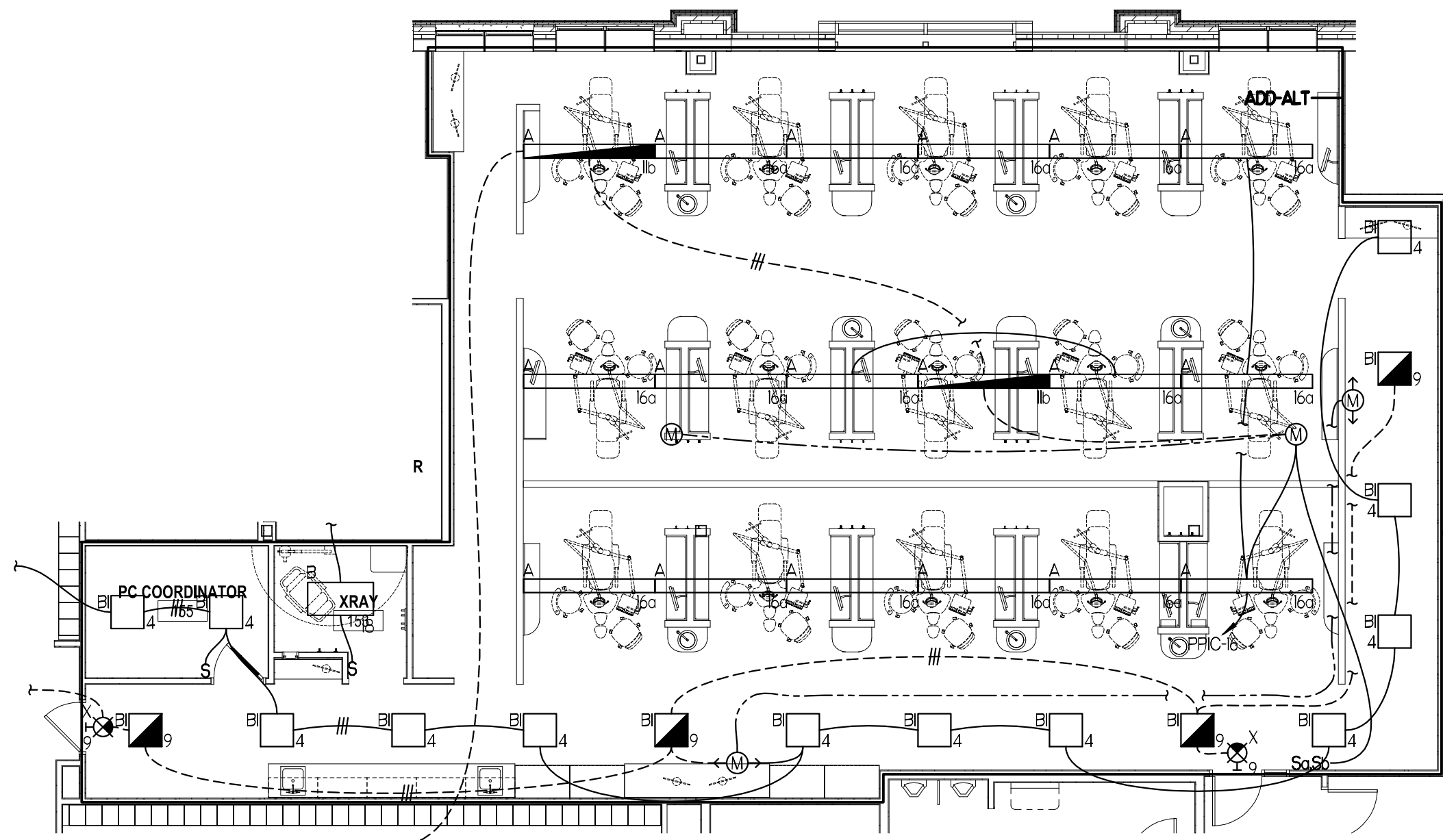
ADD ALTERNATE COMP CARE I PART PLAN SCALE: 1/8"=1'-0"
